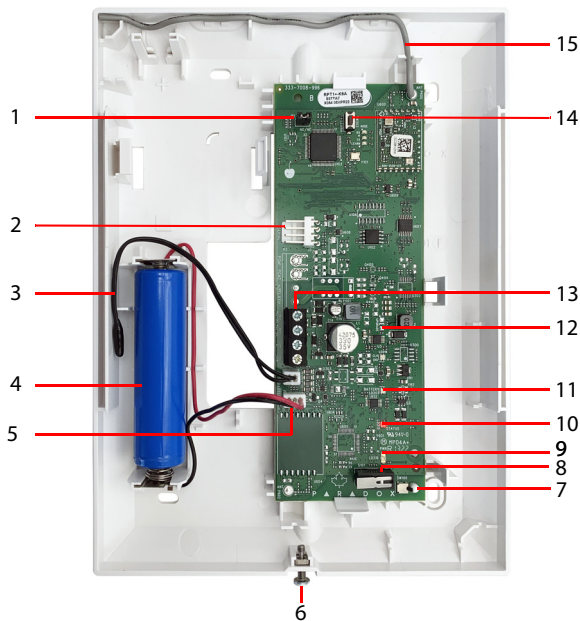
Figure 1: RPT1+ PCB
